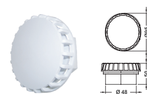
Ø2 SECTION DRAIN STRAIGHT BODY
